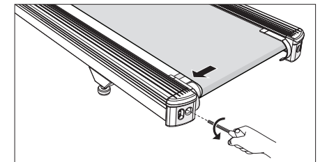
BELT IS TOO FAR TO THE RIGHT SIDE
